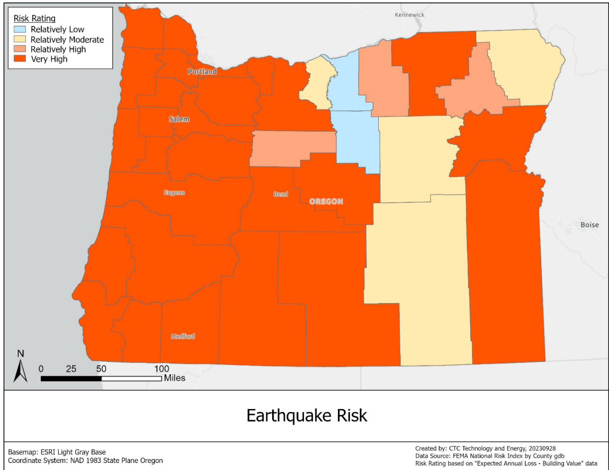
Figure 15: Map of earthquake risk in Oregon
